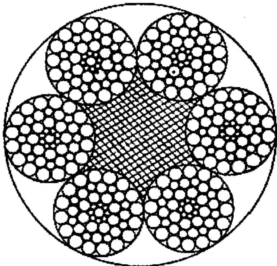
6×49SWS+FC
