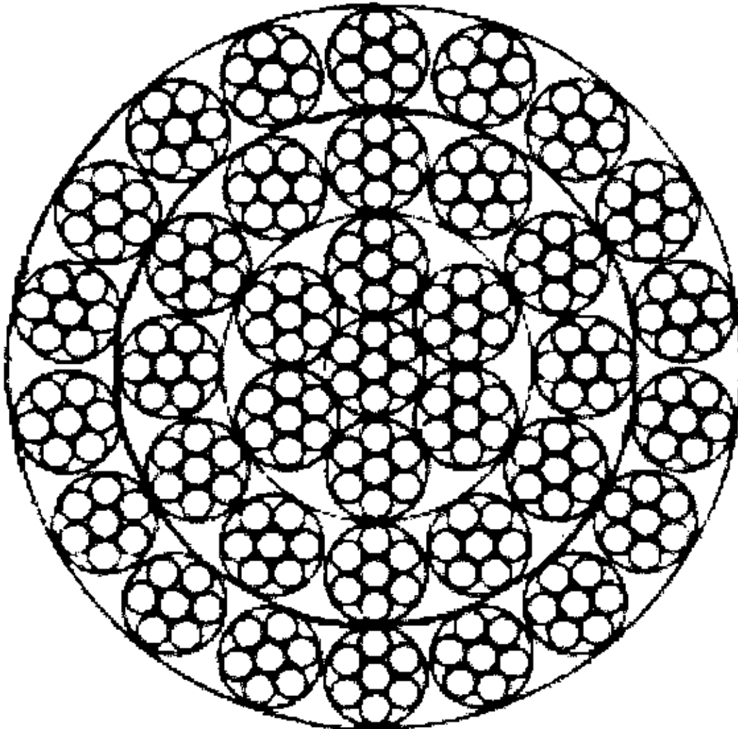
36×7+IWS
